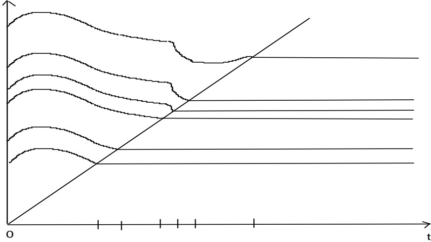
Figure 1: Sample trajectory of the flow t \mapsto (T_k^{0,t})_{k \geq 1} .
